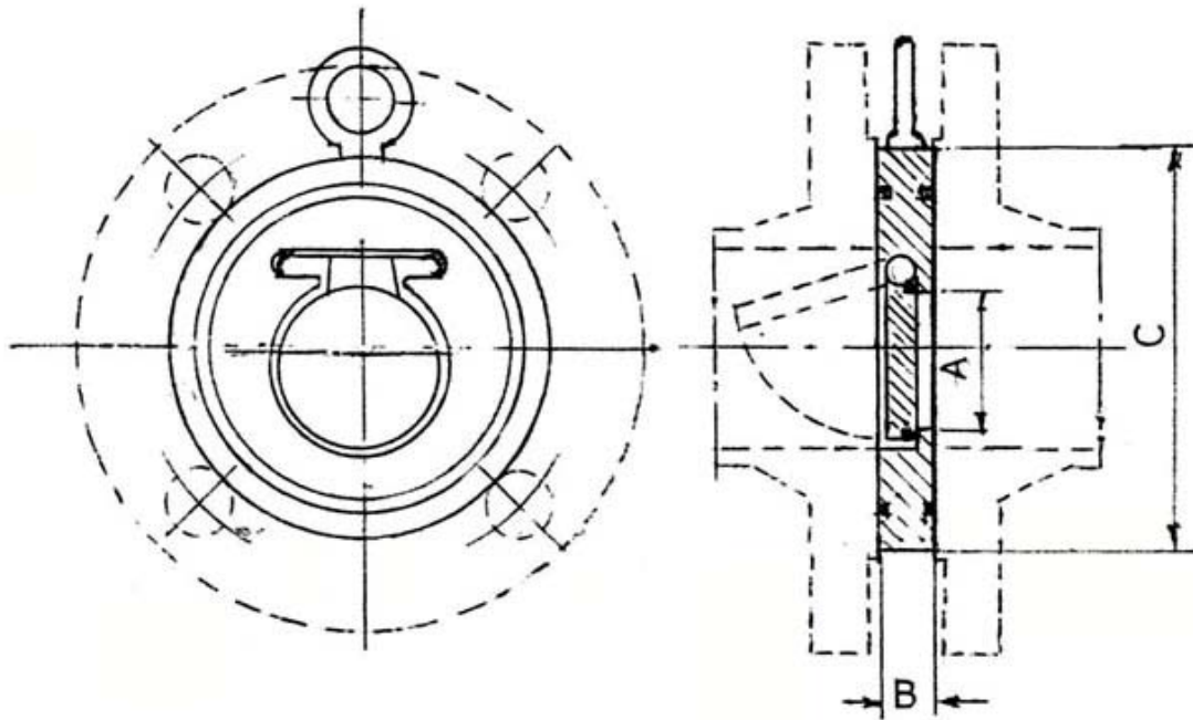
Wafer Type Check Valve (NRV)
